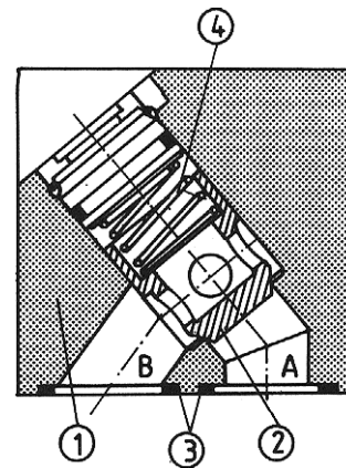
Item 3 - O-ring 29.2 × 3 - 2 pieces
